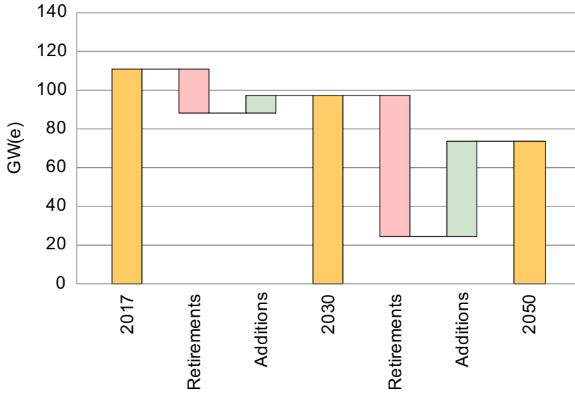
FIGURE 25. NUCLEAR CAPACITY IN THE COMBINED REGIONS OF NORTHERN, WESTERN AND SOUTHERN EUROPE: ACTUAL, RETIREMENTS AND ADDITIONS
