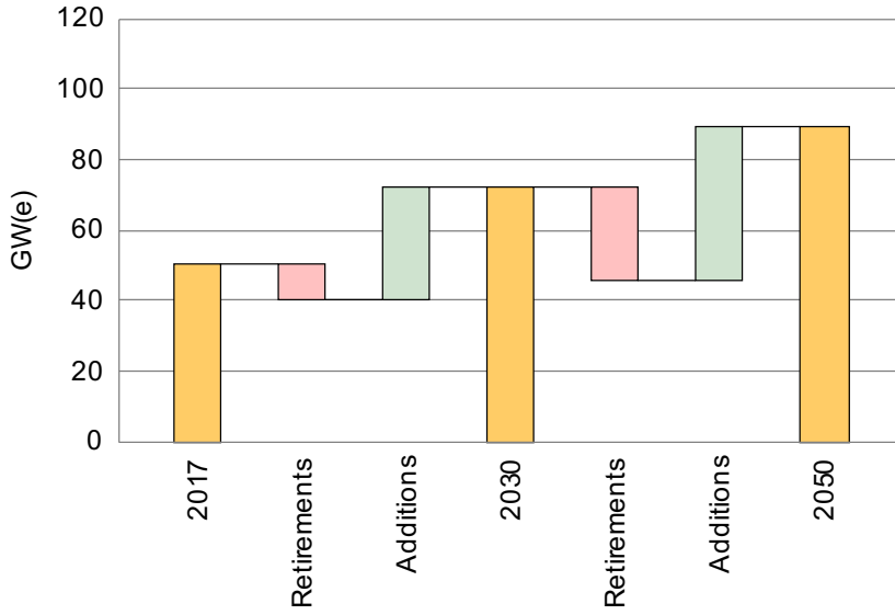
FIGURE 31. NUCLEAR CAPACITY IN THE EASTERN EUROPE REGION: ACTUAL, RETIREMENTS AND ADDITIONS
